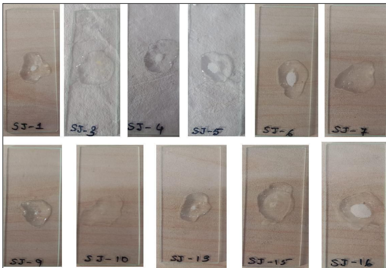
Fig 8: Observed photos of catalase test2
