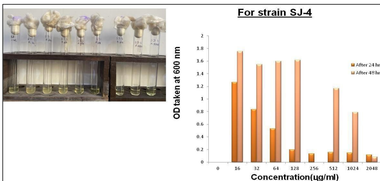
Fig 19: MIC for SJ-4
