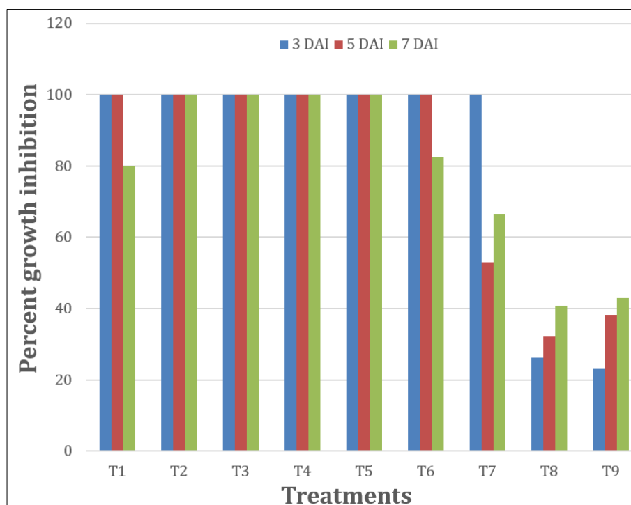
Fig 1: Effect of fungicides on per cent growth inhibition of Colletotrichum capsici
