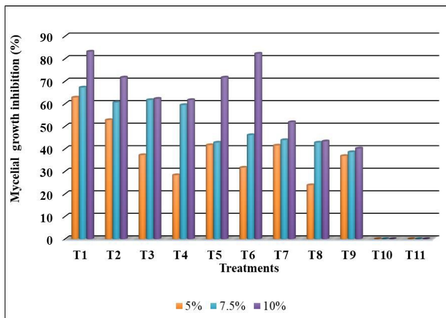
Fig 1: Evaluation of phytoextracts against C. gloeosporioides in vitro
