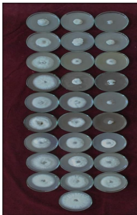
Plate 1: Evaluation of phytoextracts against C. gloeosporioides in vitro
