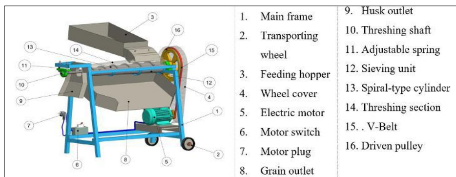
Fig 1: Finger Millet Thresher
