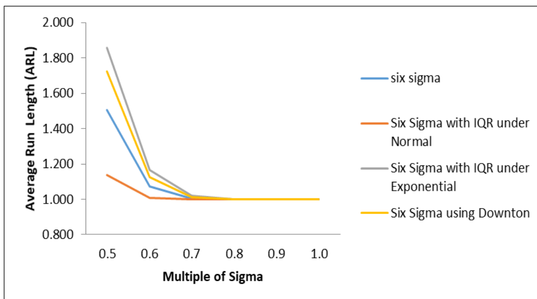
Fig 4: ARL for moving range six-sigma control charts
