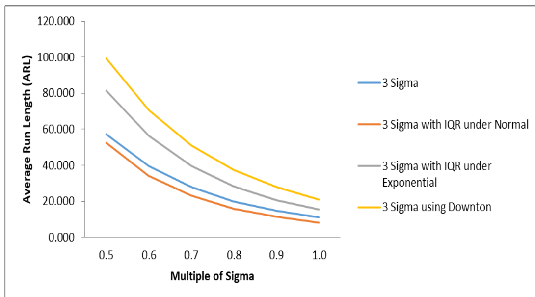
Fig 3: ARL for moving range three-sigma control charts
