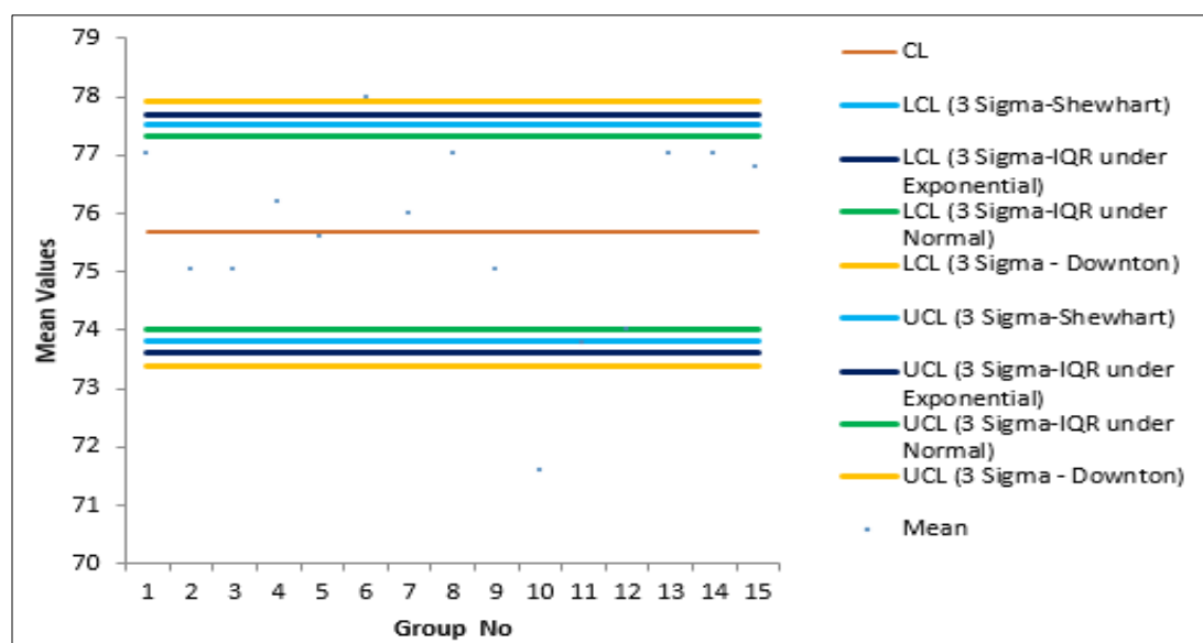
Fig 1: Three-sigma control charts for moving range
