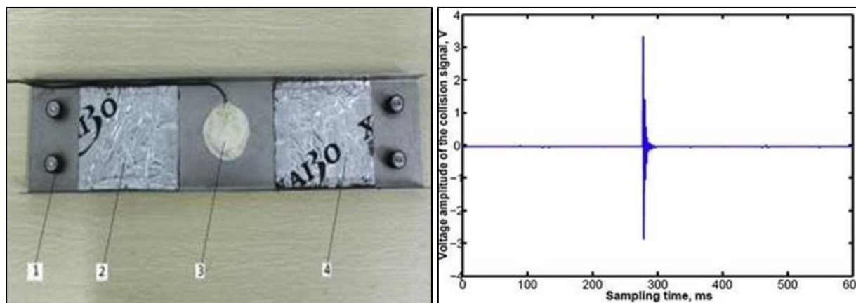
Fig 7: Optimal position of damping layer and collision signal waveform. 1. Rubber shock absorber, 2. Viscoelastic material layer 1, 3. Piezoelectric ceramic, 4. Viscoelastic material layer
