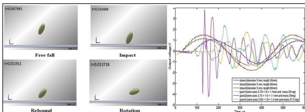
Fig 12: Typical experimental results of rice grain and MOG collision with the sensor (Alizadeh, 2013) [2]
