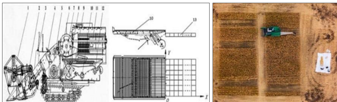
Fig 1: The harvesting machine used for the field harvesting
