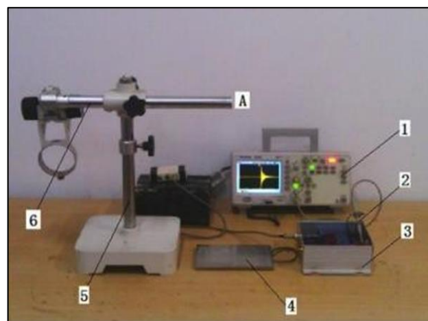
Fig 9: Single grain impact experimental system. A. Grain release point, 1. Storage digital oscilloscope, 2. Probe, 3. Signal processing circuit, 4. Grain loss sensor, 5. Support bar, 6. Height adjustment bar
