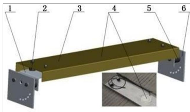
Fig 8: Structure of grain loss monitoring sensor, 1. Support plate, 2. Rubber shock absorber, 3. Sensitive plate, 4. Circular piezoelectric ceramics 5. Rubber shock absorber 2, 6. Rack connection par
