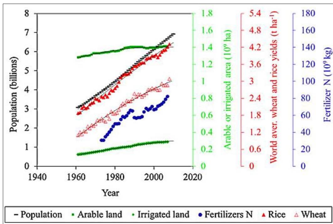
Fig 1: Evolution of population, arable land area, world average wheat and rice yields, fertilizer N use and irrigated area between 1960 and 2010 Source: (Van Ittersum, 2011) [15]
