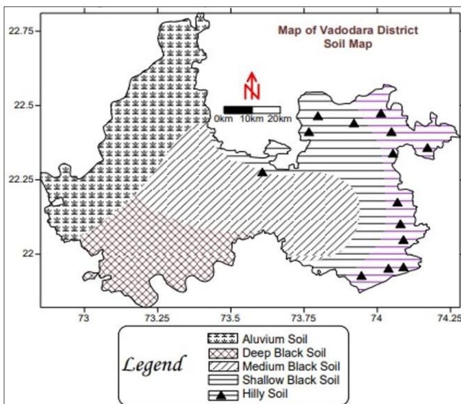
Fig 4: Soil Map of Vadodara district (Gupte, 2011) [6]
