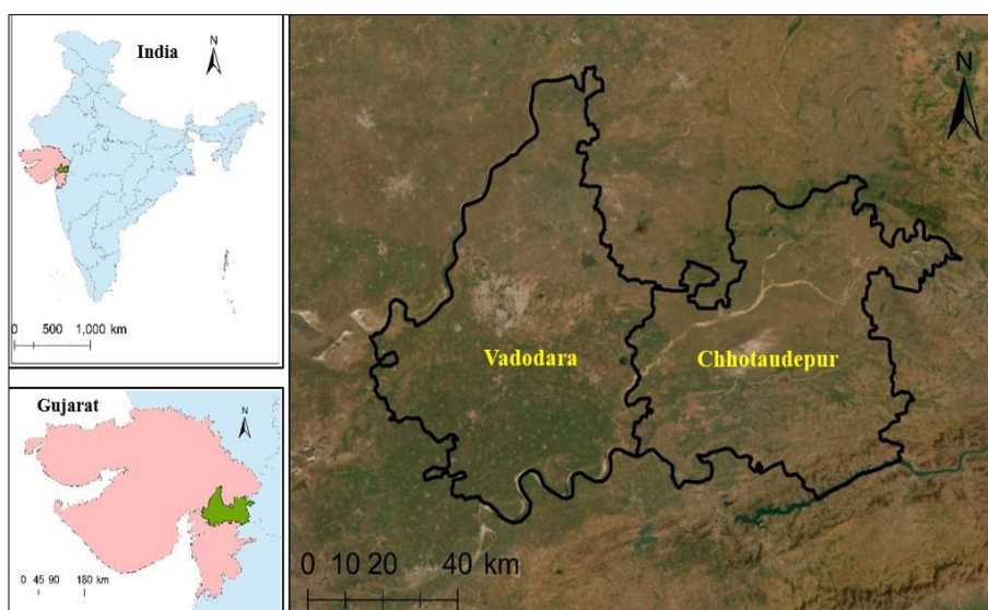
Fig 2: Map of study area India
