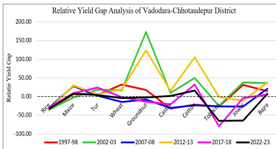
Fig 5: Relative Yield Gap analysis of Vadodara-Chhotaudepur district
