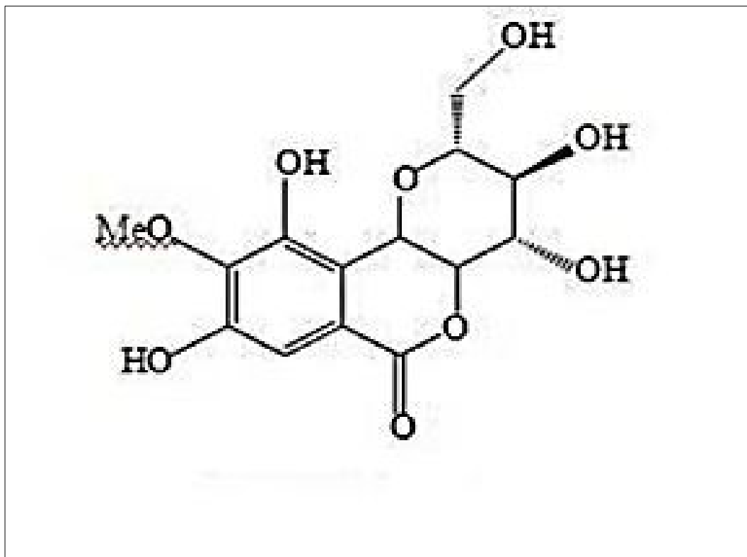
Fig 7: Bergenin
