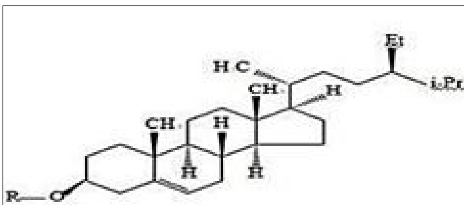
Fig 6: Sitosterol
