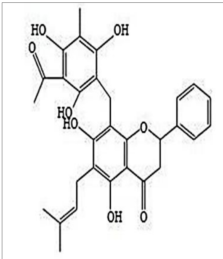
Fig 16: Isoallorottlerin
