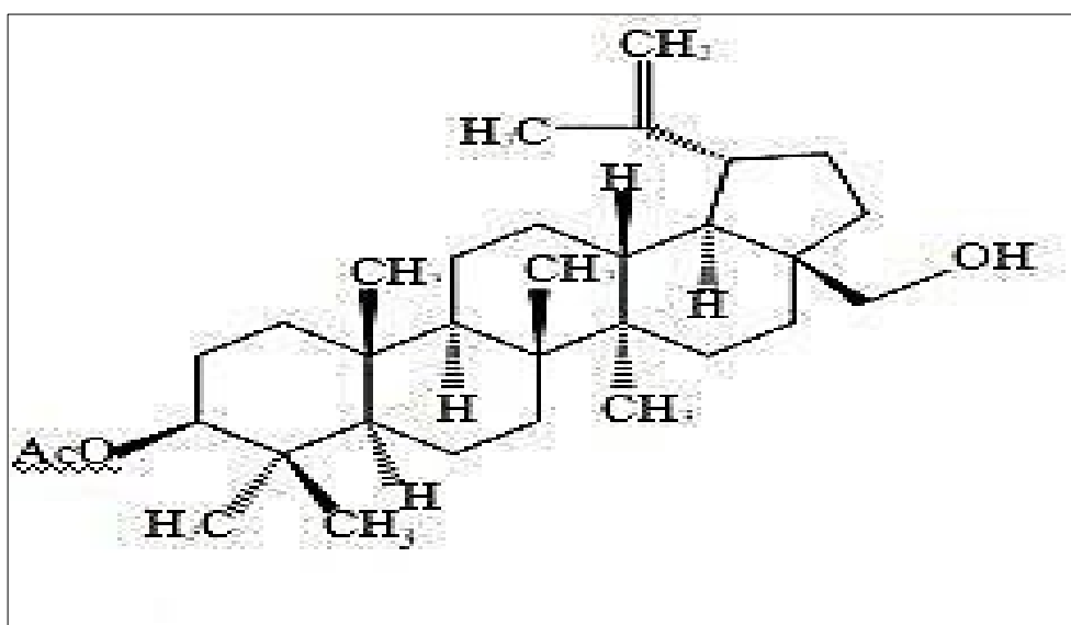
Fig 1: Betulin-3-Acetate
