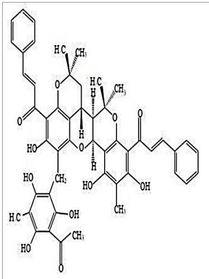
Fig 9: Kamalachalcone B
