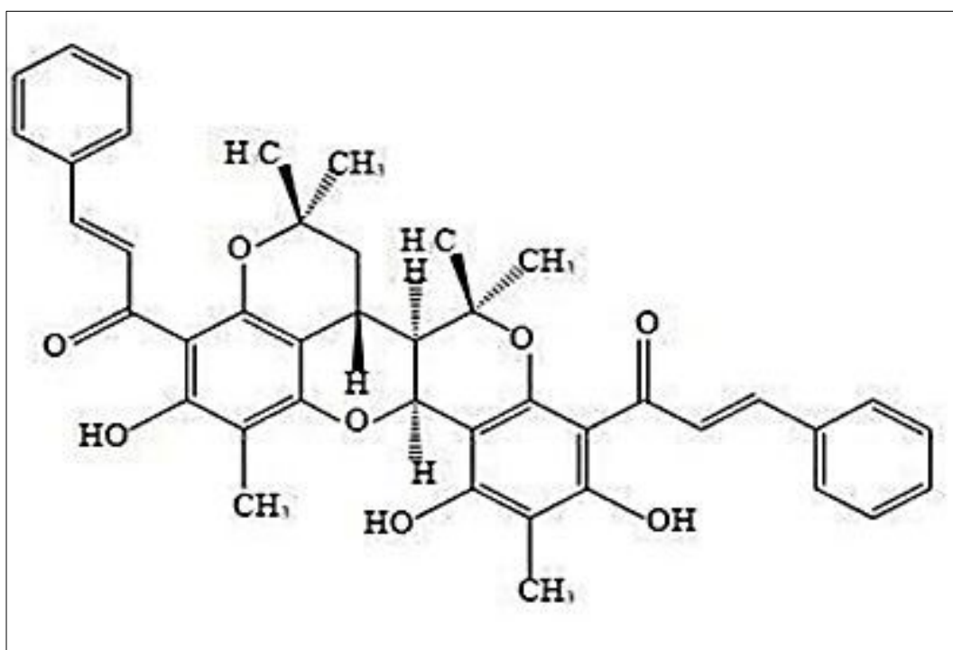
Fig 8: Kamalachalcone A
