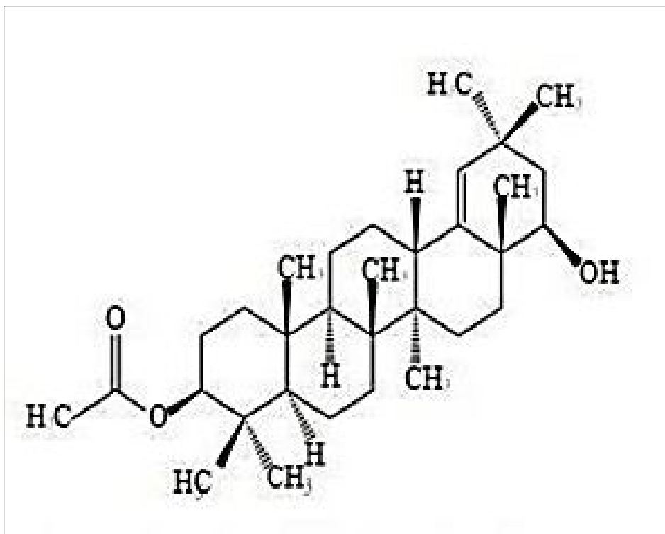
Fig 4: Acetoxy-22B-Hydroxyolean-18-ene
