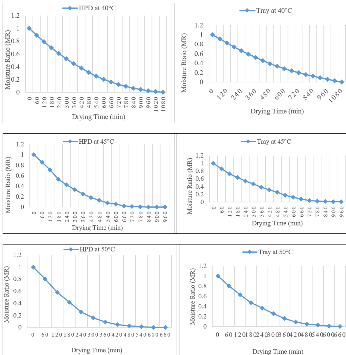
Fig 4: Plot of moisture ratio (MR) with drying time at 40°C, 45°C and 50°C temperature in heat pump drying and tray drying mode
