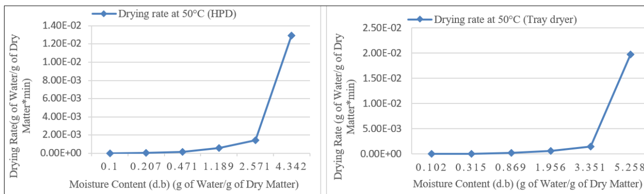
Fig 5: Plot of drying rate (DR) with moisture content (d.b) at 50°C temperature in heat pump drying and tray drying mode
