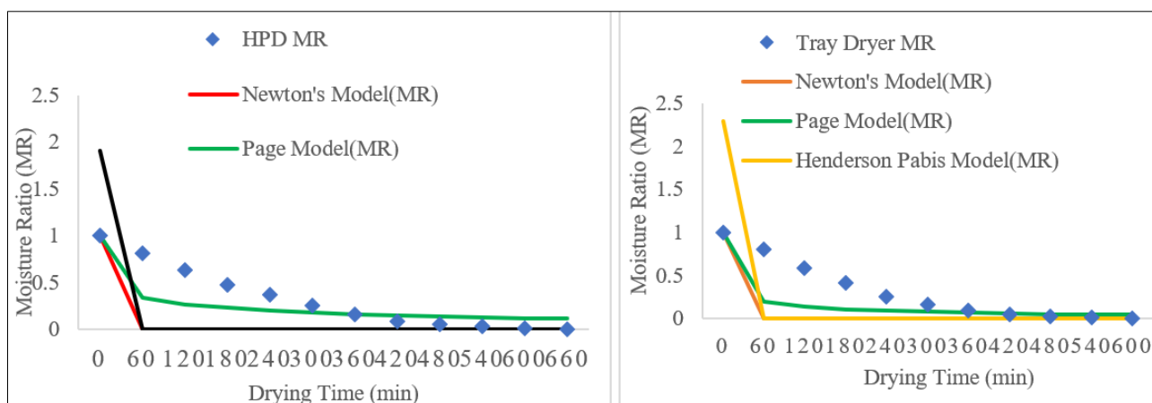
Fig 6: Fitting Newton's model, Page model and Henderson-Pabis model to the experimental data for guava dried at 50°C temperatures in HPD and tray drying mode
