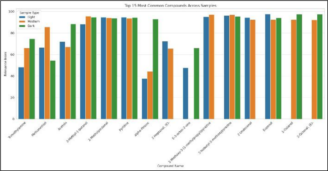
Fig 7: Common Volatile Chemical compounds across different Roast profiles of Indian Arabica Parchment
