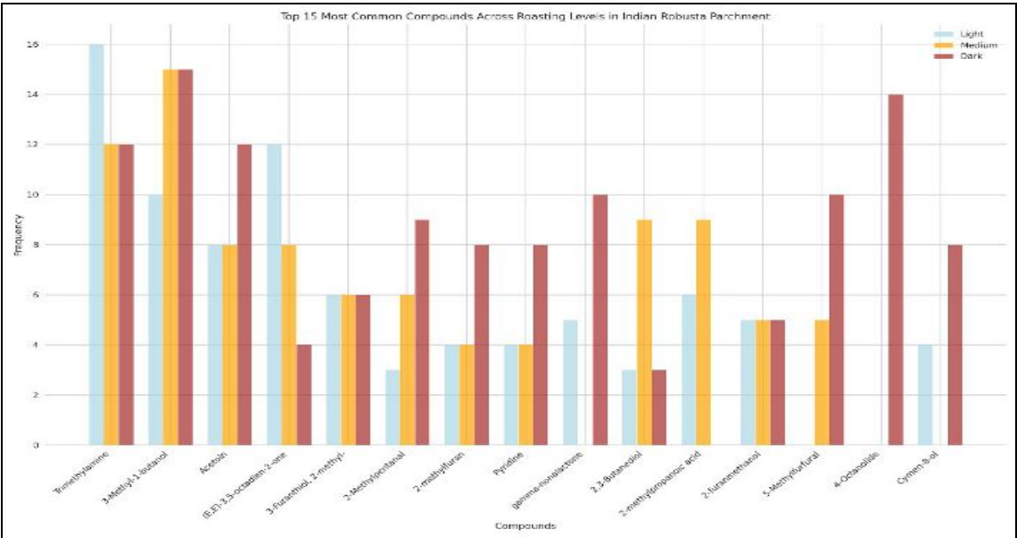
Fig 9: Common Volatile Chemical compounds across different Roast profiles of Indian Robusta Parchment
