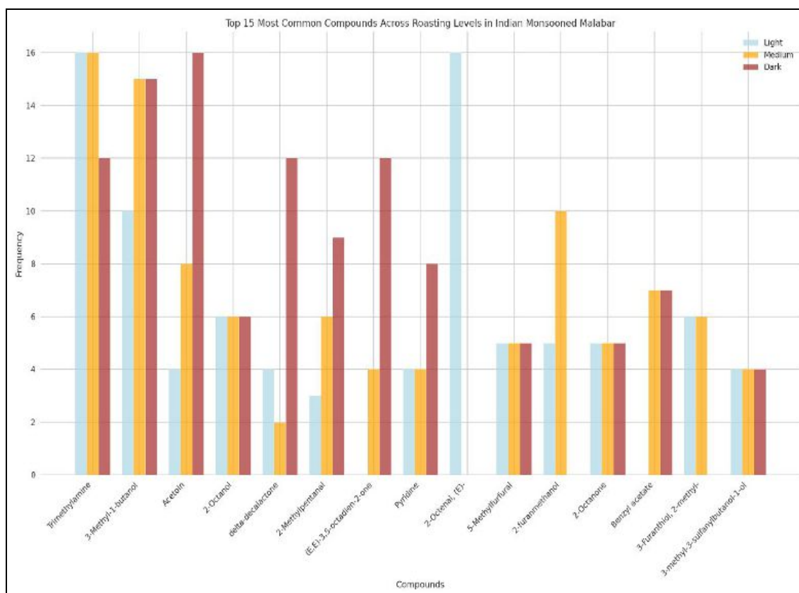
Fig 11: Common Volatile Chemical compounds across different Roast profiles of Indian Monsooned Malabar
