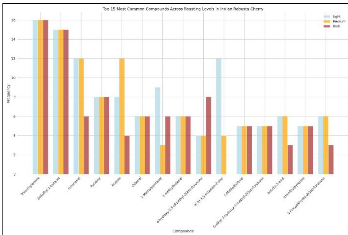
Fig 10: Common Volatile Chemical compounds across different Roast profiles of Indian Robusta Cherry
