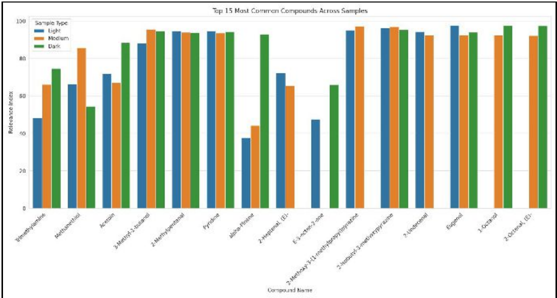
Fig 8: Common Volatile Chemical compounds across different Roast profiles of Indian Arabica Cherry
