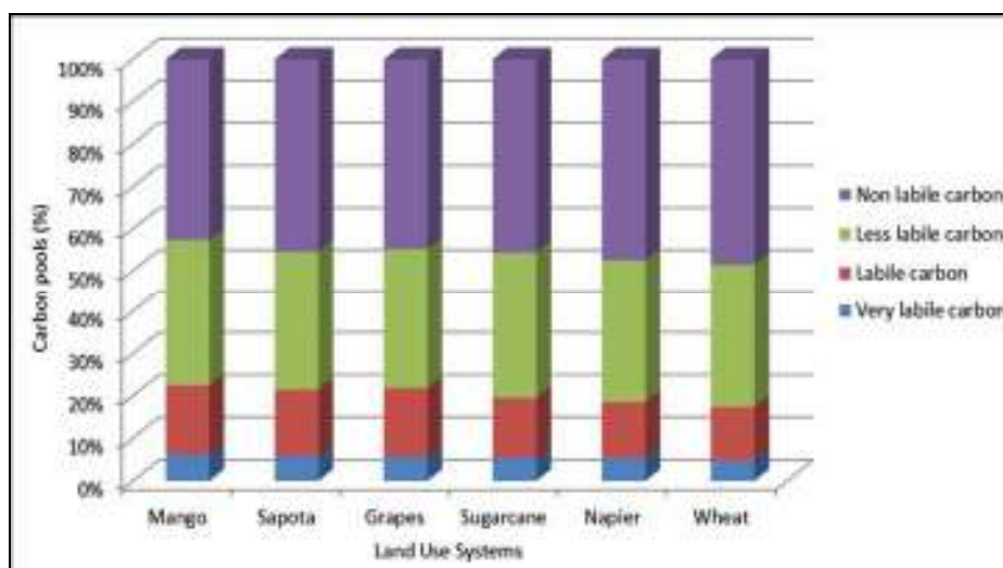
Fig 1: Percent contribution of soil organic carbon pools in different land use systems
