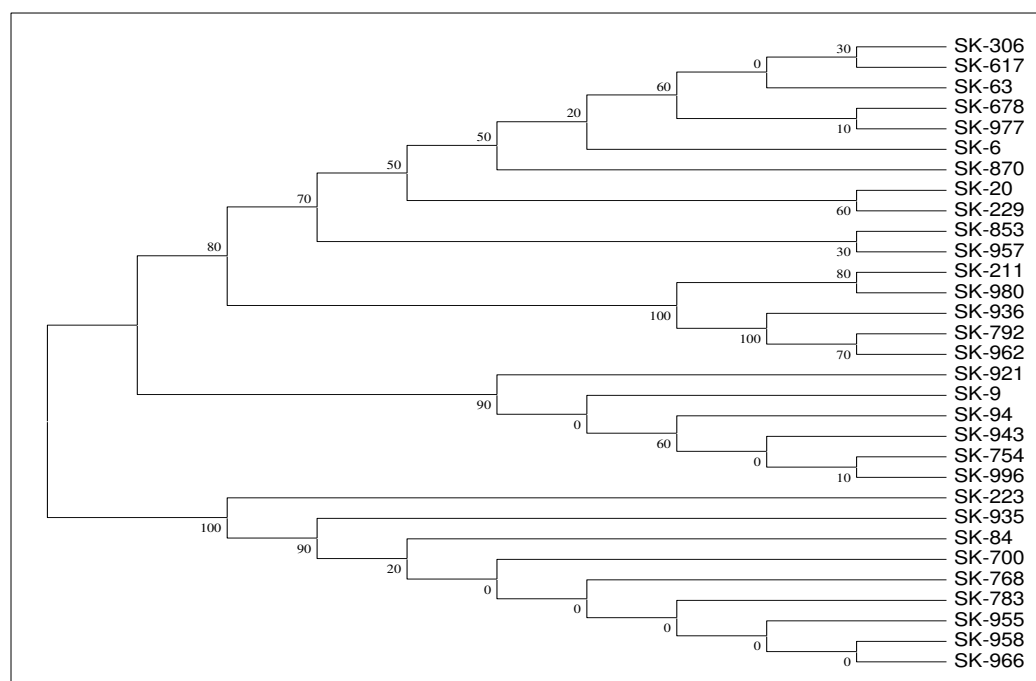
Fig 5: Phylogenetic tree showing genetic diversity of Indian Bt isolates based on 16S rRNA sequencing
