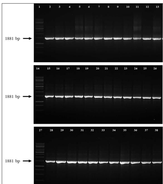
Fig 2: Gel electrophoresis of PCR-amplified 16S rRNA gene products, showing expected band size of 1881 bp from Bt isolates. Lane 1, 14, and 27: 1 Kb DNA ladder. Bt strains used as reference: in Lane 2 (HD1), Lane 15 (HD22), and Lane 28 (4G6). Lanes 3 to 13 correspond to Bt isolates SK-6, SK-9, SK-20, SK-63, SK-84, SK-94, SK-211, SK-223, SK-229, SK-306, and SK-617. Lanes 15 to 26 include Bt isolates SK-678, SK-700, SK-754, SK-768, SK-783, SK-792, SK-853, SK-870, SK-921, SK-935, and SK-936. Lanes 28 to 38 represent Bt isolates SK-943, SK-955, SK-957, SK-958, SK-962, SK-966, SK-977, SK-980, SK-996, and SK-997, respectively.
