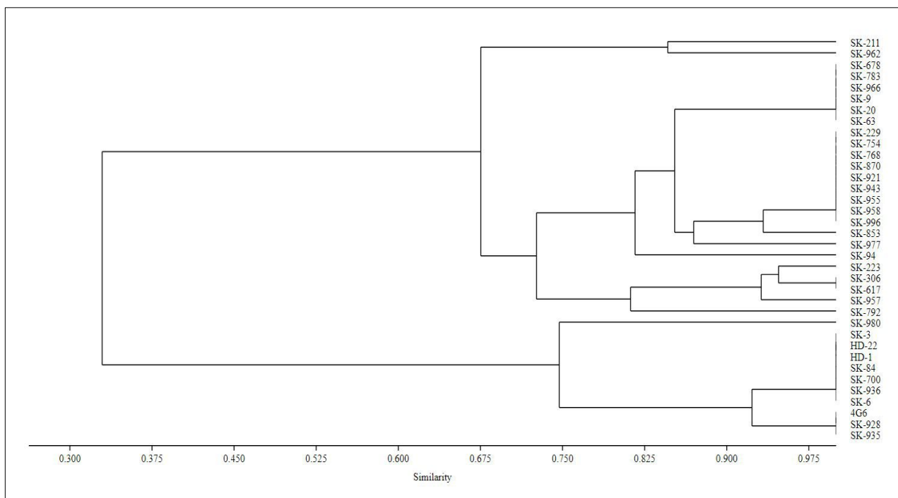
Fig 4: Dendrogram showing genetic diversity based on ARDRA pattern of 33 Indian Bt isolates and three Bt reference strains
