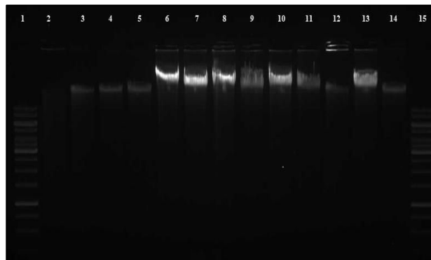
Fig 1: Agarose gel electrophoresis of isolated genomic DNA from Bt isolates, showing high molecular weight bands. Lane 1 and Lane 15 shows 1 kb DNA marker (MBI Fermentas, Germany) and the remaining Lanes depict Bt isolates
