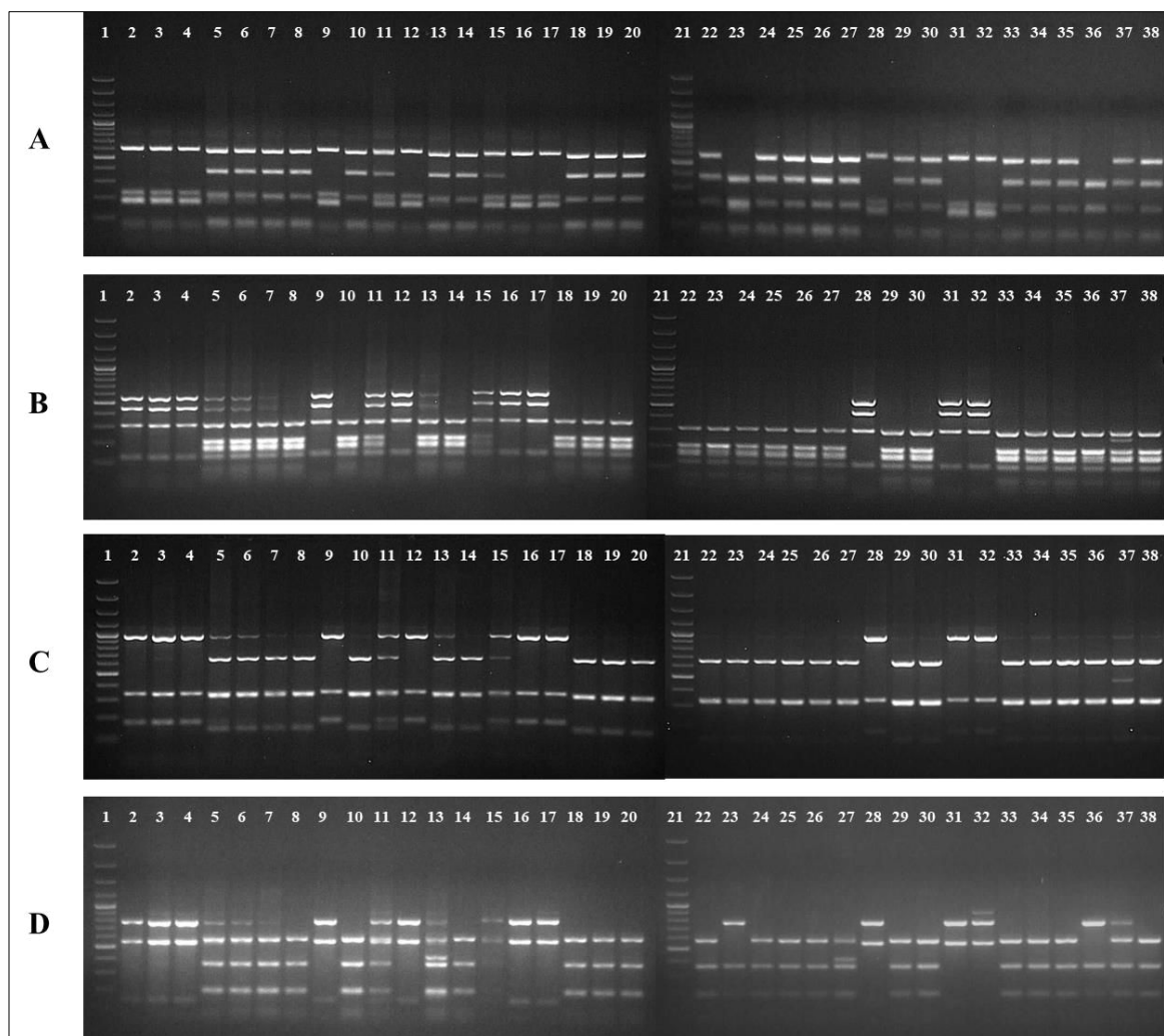
Fig 3: Banding patterns after restriction digestion of 16S rDNA amplified product with four restriction enzymes A) AluI , B) HaeIII , C) HinfI , and D) TaqI . Showing distinct fragment patterns corresponding to each enzyme's specific cleavage site. Lane 1 and 2 from each image shows 100 bp Pluse DNA marker (MBI Fermentas, Germany). Lane 2 to 20 depicts HD1, SK-3, SK-84, SK-223, SK-306, SK-617, SK-678, SK-700, SK-783, SK-792, SK-936, SK-957, SK-966, SK-980, HD22, SK-6, SK-9, SK-20, and SK-63 respectively. Lane 22 to 38 depicts SK-94, SK-211, SK-229, SK-754, SK-768, SK-853, 4G6, SK-870, SK-921, SK-928, SK-935, SK-943, SK-955, SK-958, SK-962, SK-977, and SK-996 respectively.
