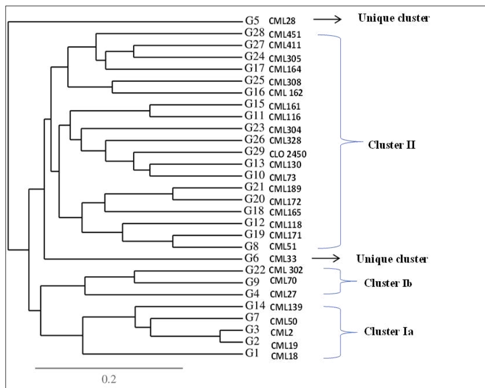
Fig 2: Dendrogram of 29 maize genotypes developed on the basis of polymorphism revealed by the 13 SSR markers.
