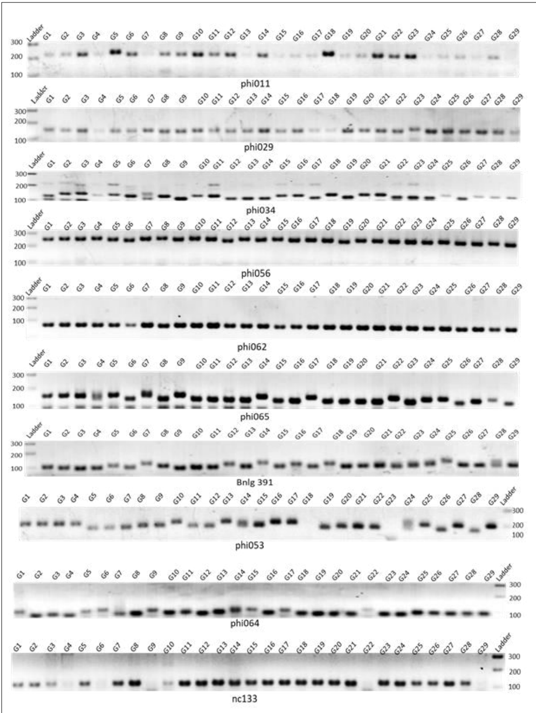
Fig 1: PCR amplification using SSR primers - phi011, phi029, phi034, phi056, phi065 bnlg391, phi014 phi032, phi053, phi064 &nc133 in twenty nine maize genotypes.
