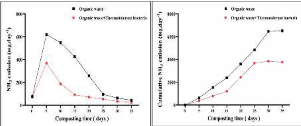
Fig 4: Impact of thermotolerant bacterial inoculation on ammonia (NH 3 ) emissions during composting. (A) Daily ammonia emission rates reveal a significant reduction in peak emissions for the bacterial treatment compared to the control, attributed to enhanced ammonium (NH 4 + ) conversion via nitrification. (B) Cumulative ammonia emissions demonstrate the sustained nitrogen retention achieved with thermotolerant bacterial inoculation, reducing overall nitrogen losses and improving compost nitrogen efficiency.
