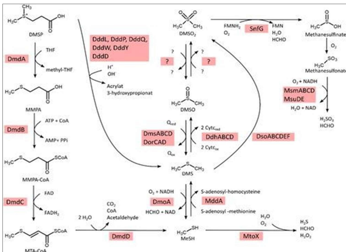
Fig 3: Prokaryotic metabolism of C1 organosulphur compounds. All proteins shown have a corresponding HMM in HMSS2. CytC, Cytochrome c; DMSP, dimethylsulphoniopropionate; DHPS, 2,3-dihydroxypropane-1-sulphonate; DMS, dimethylsulphide; DMSO, dimethylsulphone, DM
