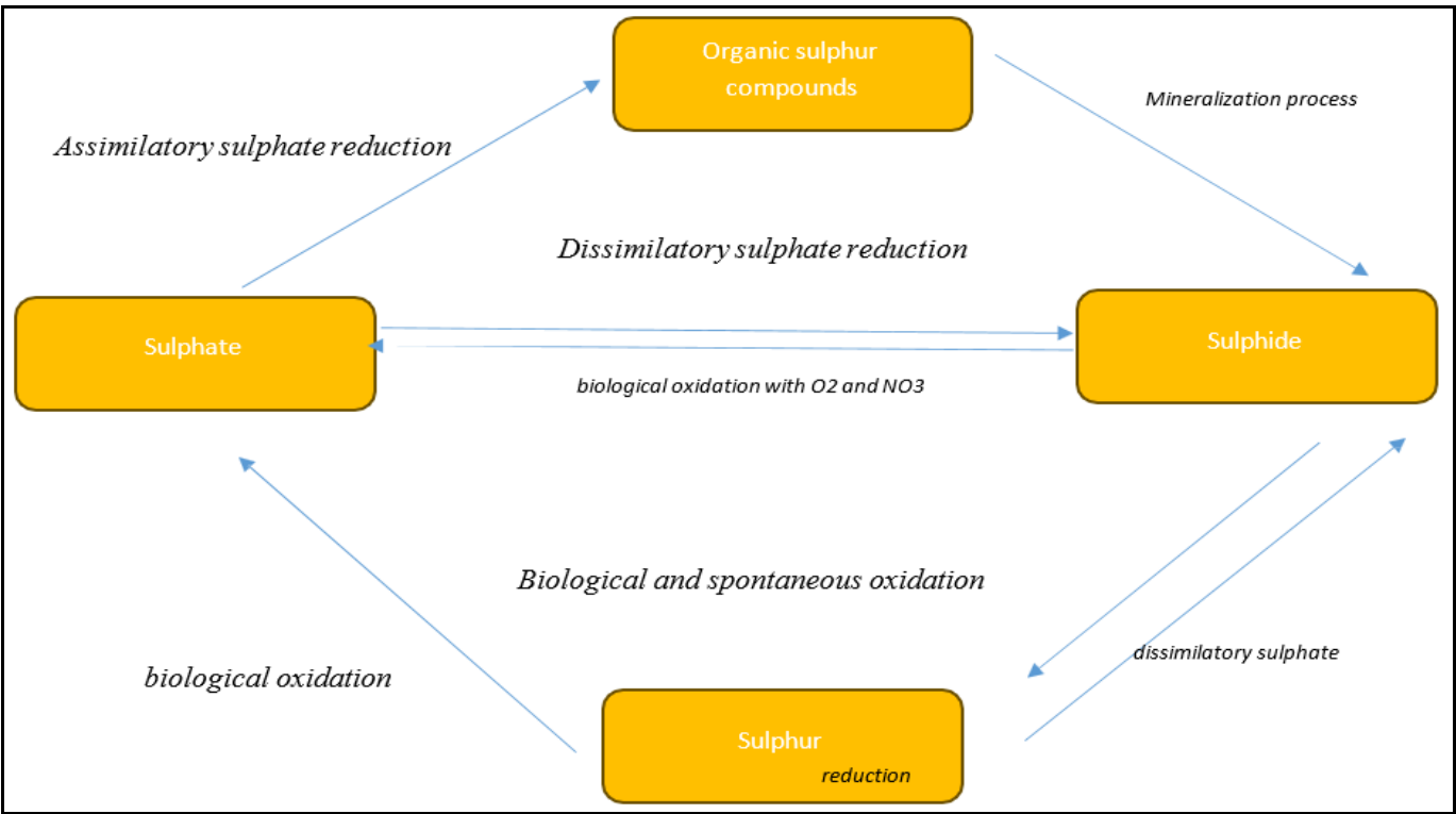
Fig 2: Biological Sulphur Cycle
