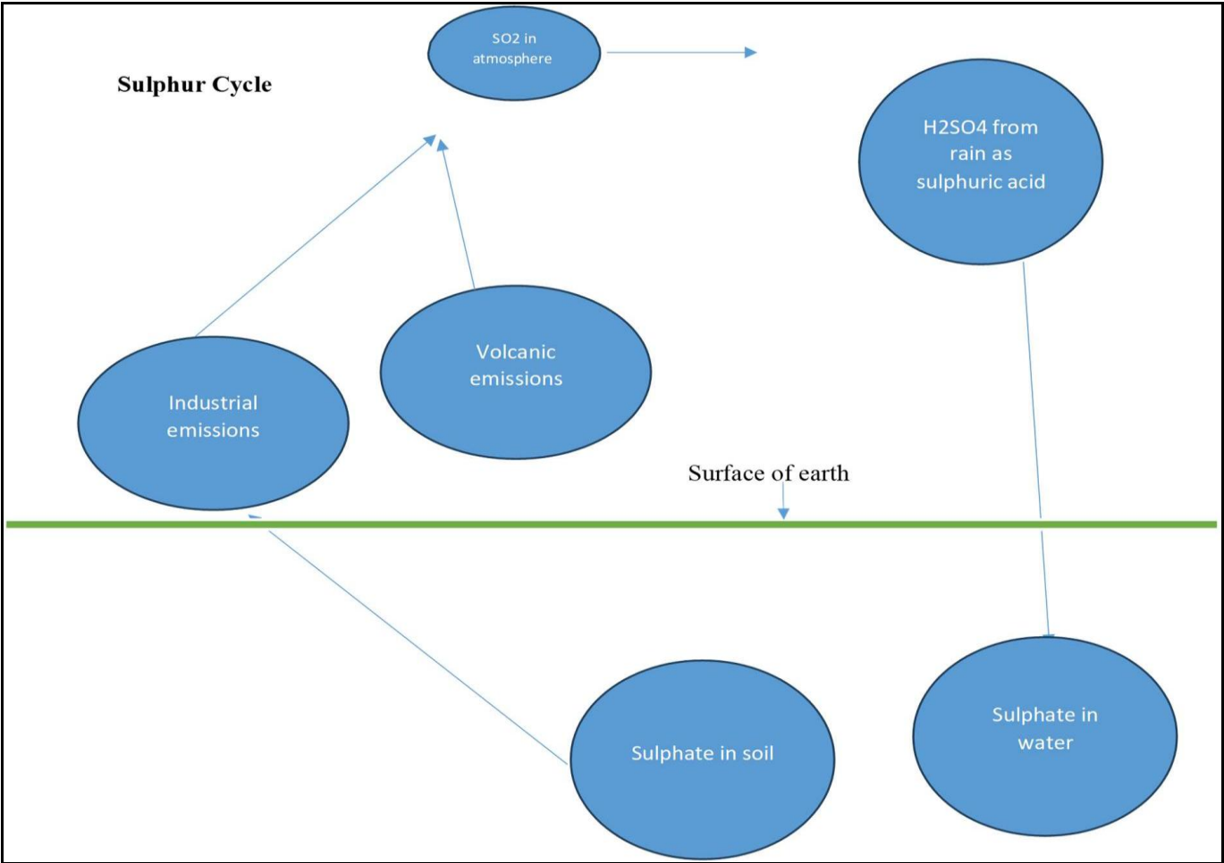
Fig 1: Sulphur cycle
