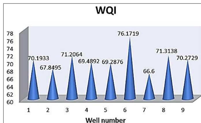
Fig 11: The WQI value for each well
