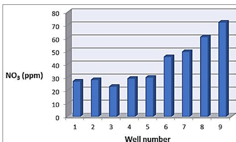
Fig 6: Nitrates ( \text{NO}_3 ) for the studied water models
