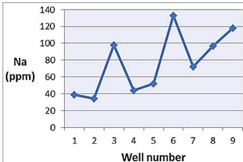
Fig 9: Sodium concentration (Na)
